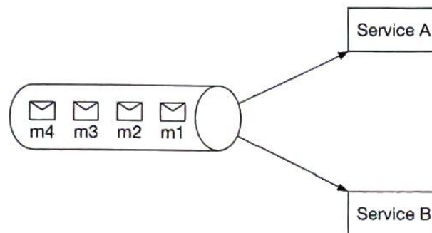
Figure 11.7: Message queue
