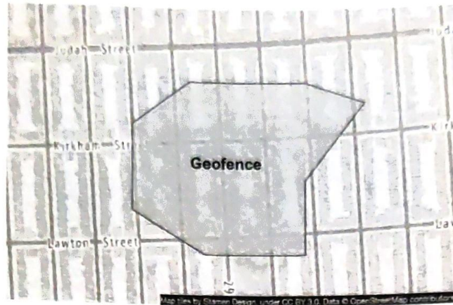
Figure 1.17: Geofence
