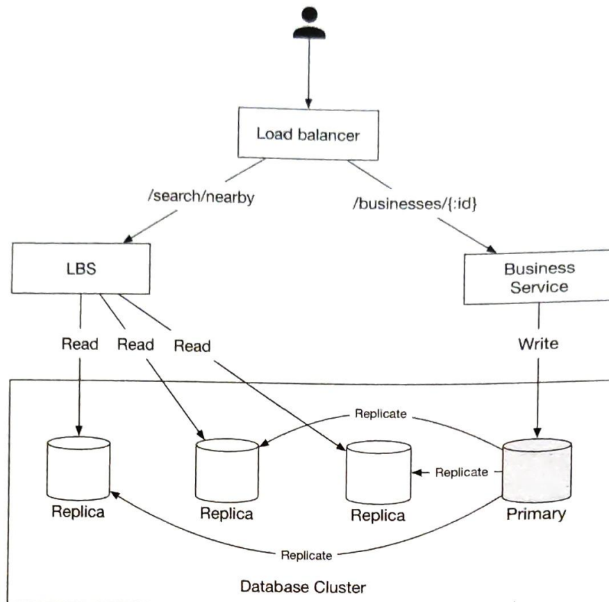
Figure 1.2: High-level design
