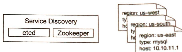
Figure 5.9: Service discovery
