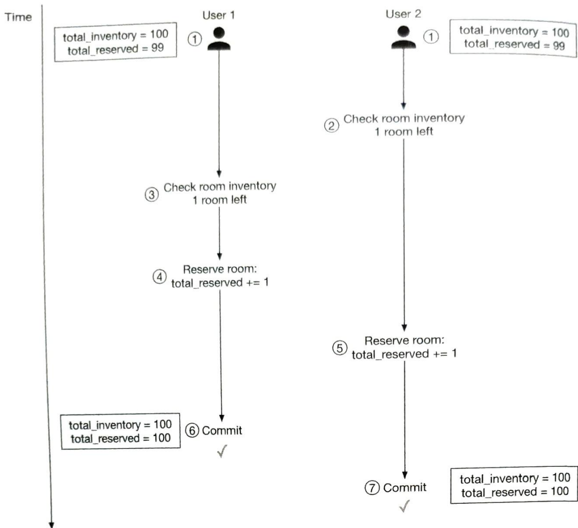
Figure 7.11: Race condition
