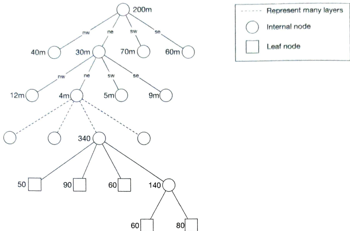
Figure 1.14: Build quadtree
