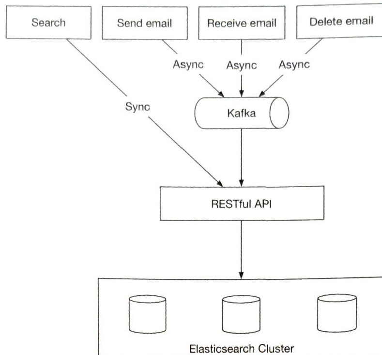
Figure 8.10: Elasticsearch
