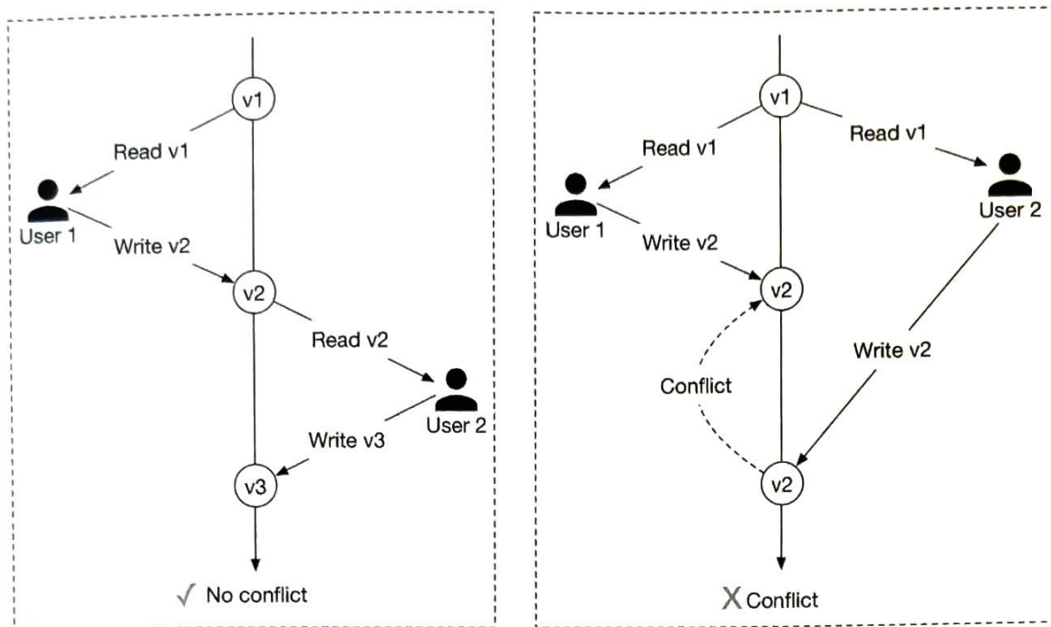
Figure 7.13: Optimistic locking
