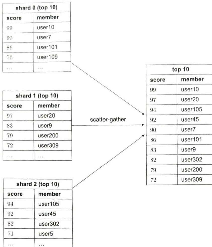
Figure 10.20: Scatter-gather
