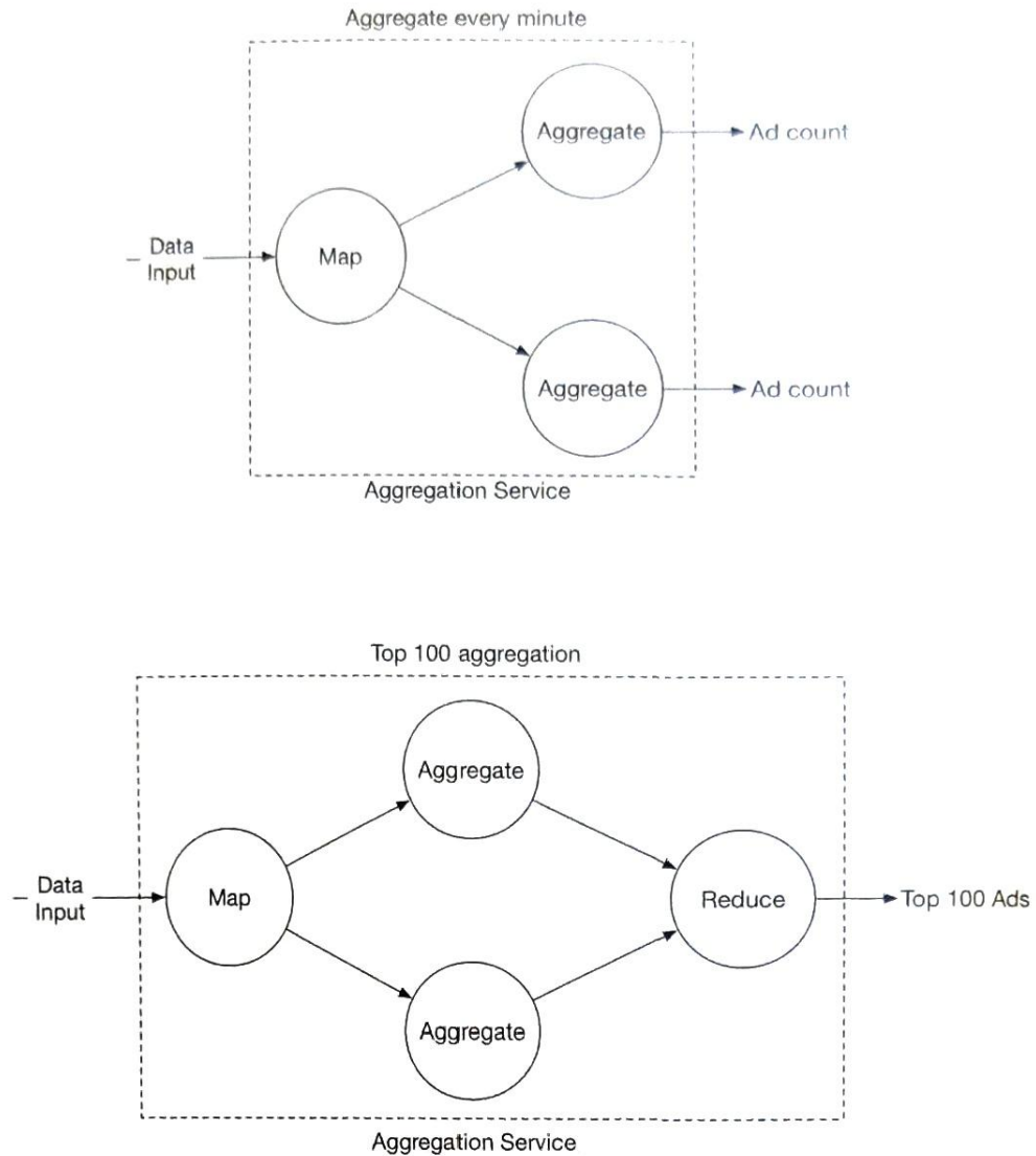
Figure 6.5: Aggregation service
