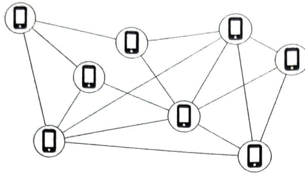
Figure 2.2: Peer-to-peer
