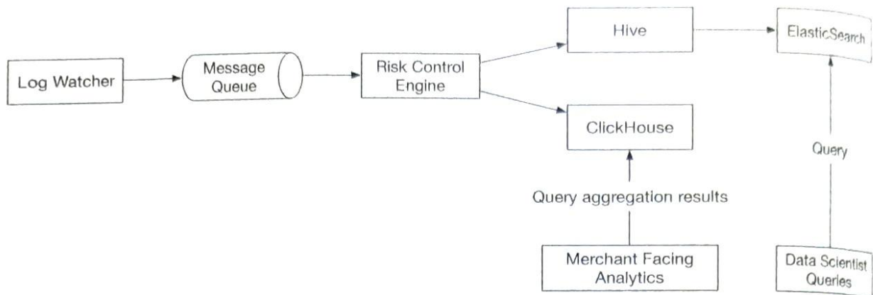
Figure 6.29: Alternative design
